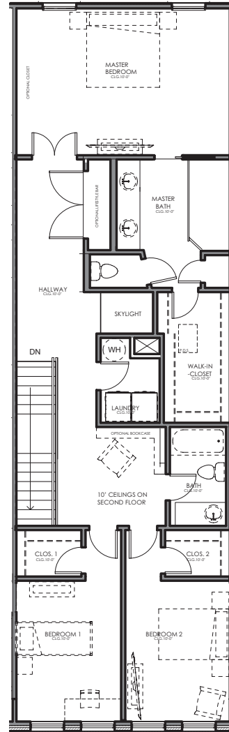
Upper Level
