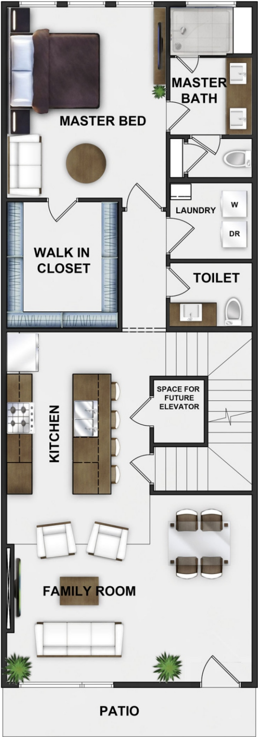
FIRST FLOOR
