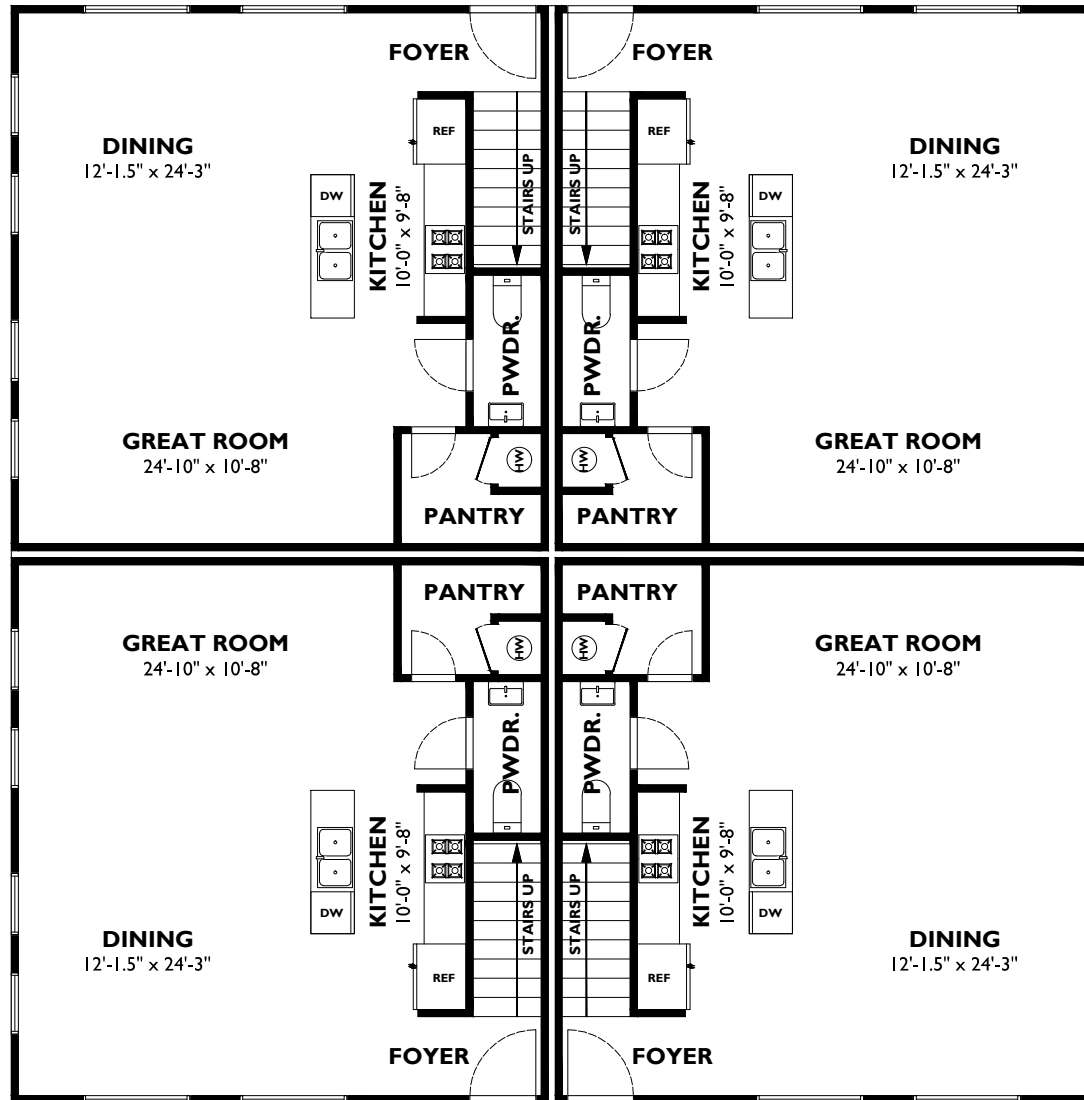
FIRST FLOOR
