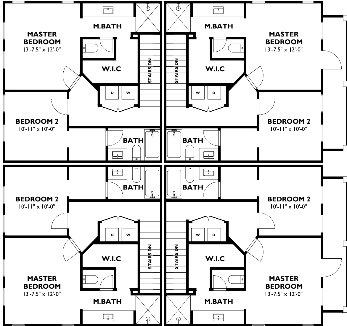
SECOND FLOOR
